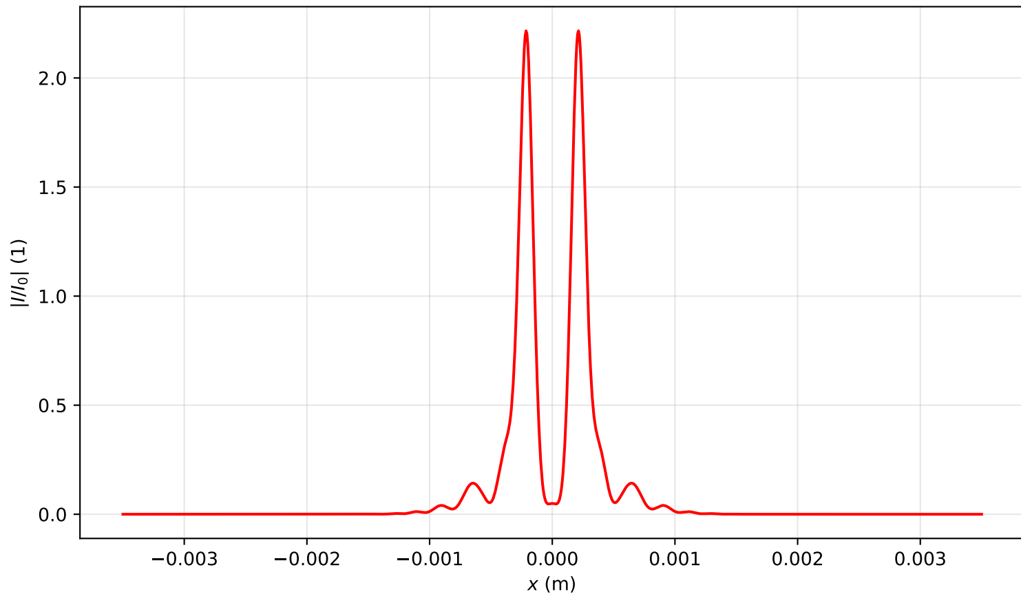
Intensity profile I(x, y = 0, z = 0.716)/I_0 , P_{in}=5.0P_{cr} , artificial time
